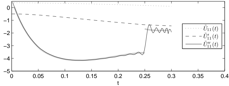
Fig. 3. The approximation \tilde{U}'' exhibits Gibbs phenomenon ( N = 50 ) since U'' (gray) is discontinuous.
