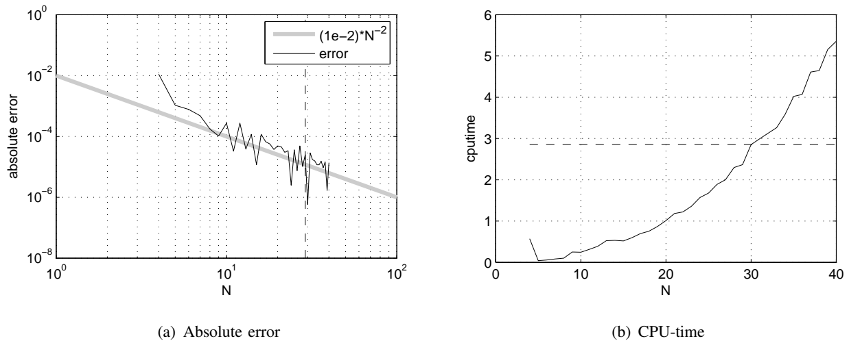
Fig. 2. Number of discretization points N vs error and CPU-time for Example 3.
