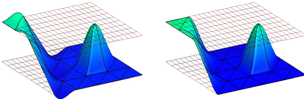
Fig. 5. Hermite interpolation versus nonnegativity preserving interpolation to function (6.3) using Clough-Tocher splines on the type-1 triangulation \Delta_1 of \Omega . The planes z = 0 and z = 1 are shown as grids.
