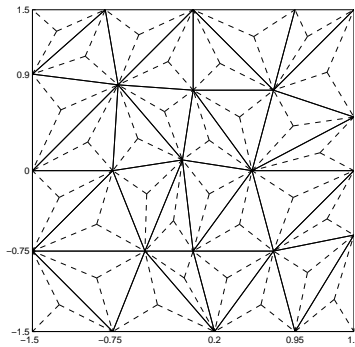
Fig. 3. A Delaunay triangulation of 25 points in the domain \Omega of Example 6.1, and the corresponding CT-refinement (indicated with dashed lines).
