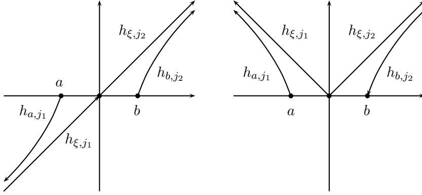
Figure 1: Contours of integration in the complex plane corresponding to even r (left) and odd r (right).
