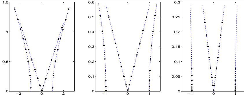
Figure 2: Location of the quadrature nodes for an oscillatory integral on [-1, 1] with r = 3 , corresponding to \omega = 1 (left), \omega = 10 (center) and \omega = 100 (right). Eight points have been computed on each contour. The points are located on the paths of steepest descent (dashed line).
