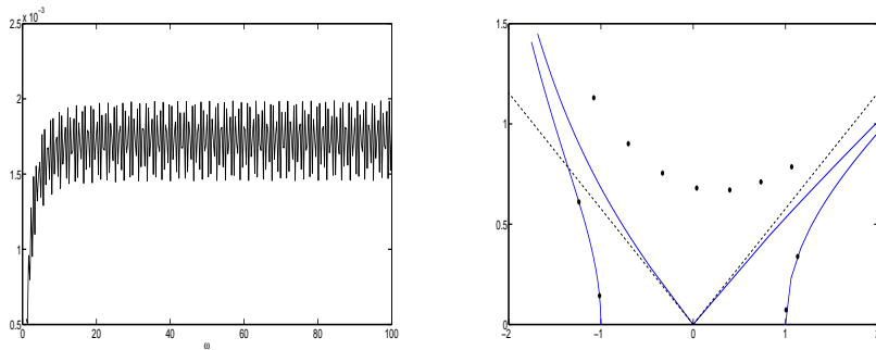
Figure 11: Absolute error in the evaluation of \int_{-1}^1 [\sin(x) + \cos(x)] e^{i\omega(x^4+4x^3)} dx . We have used 2 + 7 quadrature nodes. The left panel shows the absolute error, scaled by \omega^5 (at \omega = 100 , the error is 1.8 \times 10^{-13} ). The right panel shows the paths of steepest descent (solid lines), the paths of steepest descent for g(x) = x^3 (dashed lines) and the location of the quadrature points corresponding to \omega = 1 .
