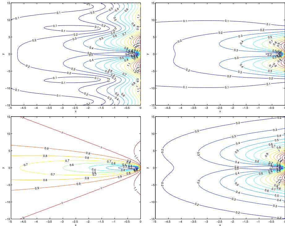
FIG. 4.1. Contour plots of the fully convergence factor \rho(\mathcal{K}(z)) with z := a\Delta T \in \mathbb{C}^- , for 4 different F -propagator - G -propagator combinations: Exact solution - backward Euler (top left), Backward Euler ( M=10 ) - backward Euler (top right), trapezoidal rule ( M=1 ) - backward Euler (bottom left), and Radau IIA ( M=1 ) - backward Euler (bottom right).
