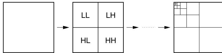
Figure 1: The two-dimensional wavelet transform: iteration on the LL subband, showing the wavelet coefficients in “Mallat” ordering.
