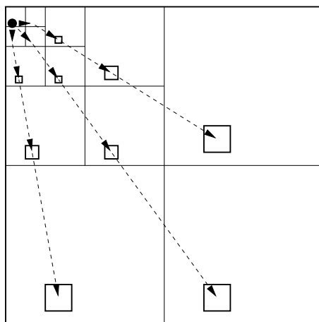
Figure 6: Zerotree compression: a tree of coefficients at different resolution levels that correspond to one low pass coefficient.
