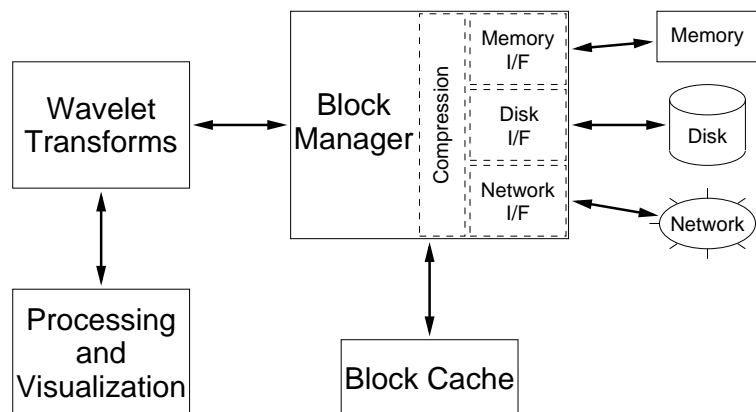
Figure 5: Design of the large scale image processing system.
