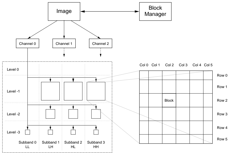
Figure 4: Subdivision of an image into channels, levels, subbands and blocks.
