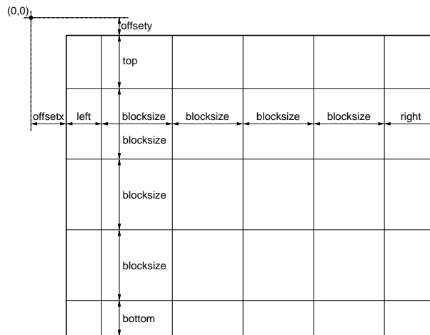
Figure 3: Division of a subband in blocks. The margins (top, bottom, left and right) are chosen such that the coordinates of the block boundaries are always multiples of the block size.
