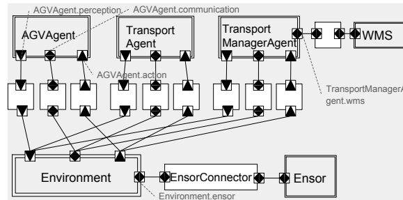
Fig. 3. Decomposition in agents and environment for AGVTS.
