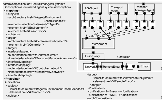
Fig. 12. Final composition in centralized agent system for AGVTS. (a) Composition specification. (b) Reification of composition.
