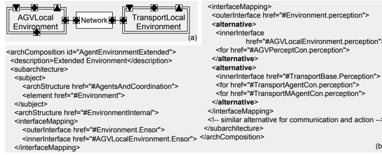
Fig. 14. (a) EnvironmentInternal structure. (b) Specification to compose EnvironmentInternal with AgentsAndCoordination.
