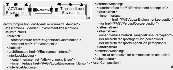
Fig. 11. (a) EnsorConnectorInternal structure. (b) Composition specification.
