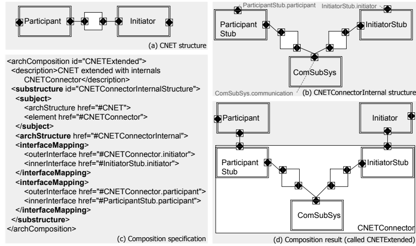
Fig. 8. (a) CNET structure. (b) CNETConnectorInternal structure. (c) Composition specification to compose CNET and CNETConnectorInternal. (d) Reification of composition, called CNETExtended.
