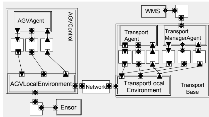
Fig. 5. First decomposition view of architectural documentation.
