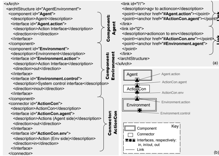
Fig. 1. Example xADL specification, showing the Agent and Environment component, connected with the ActionCon connector. We used the same abbreviated notation as the xADL authors used in [14] to improve readability of the specification. We will only once include a key, the other figures use the same graphical notation.
