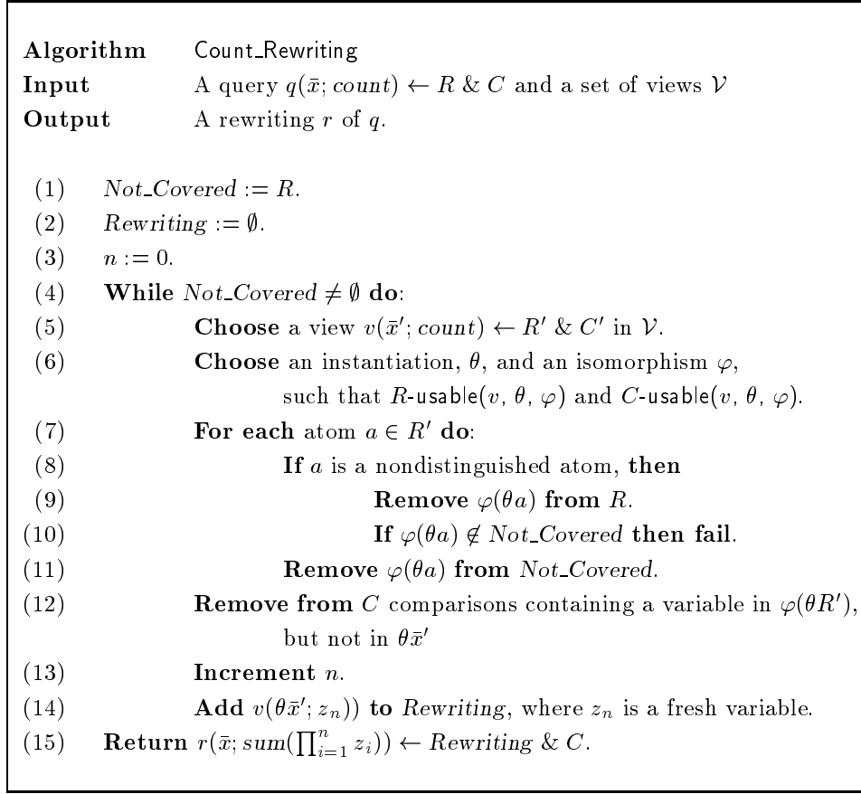
Fig. 1. Count Query Rewriting Algorithm
